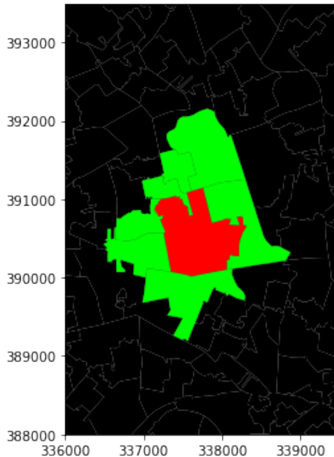
Queen neighbors of `E01006690`
